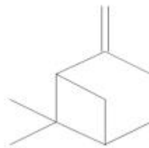
Gambar 6. Bicyclo[3.1.1]heptane, 6,6-dimethyl-2-methylene-, (1S)-
