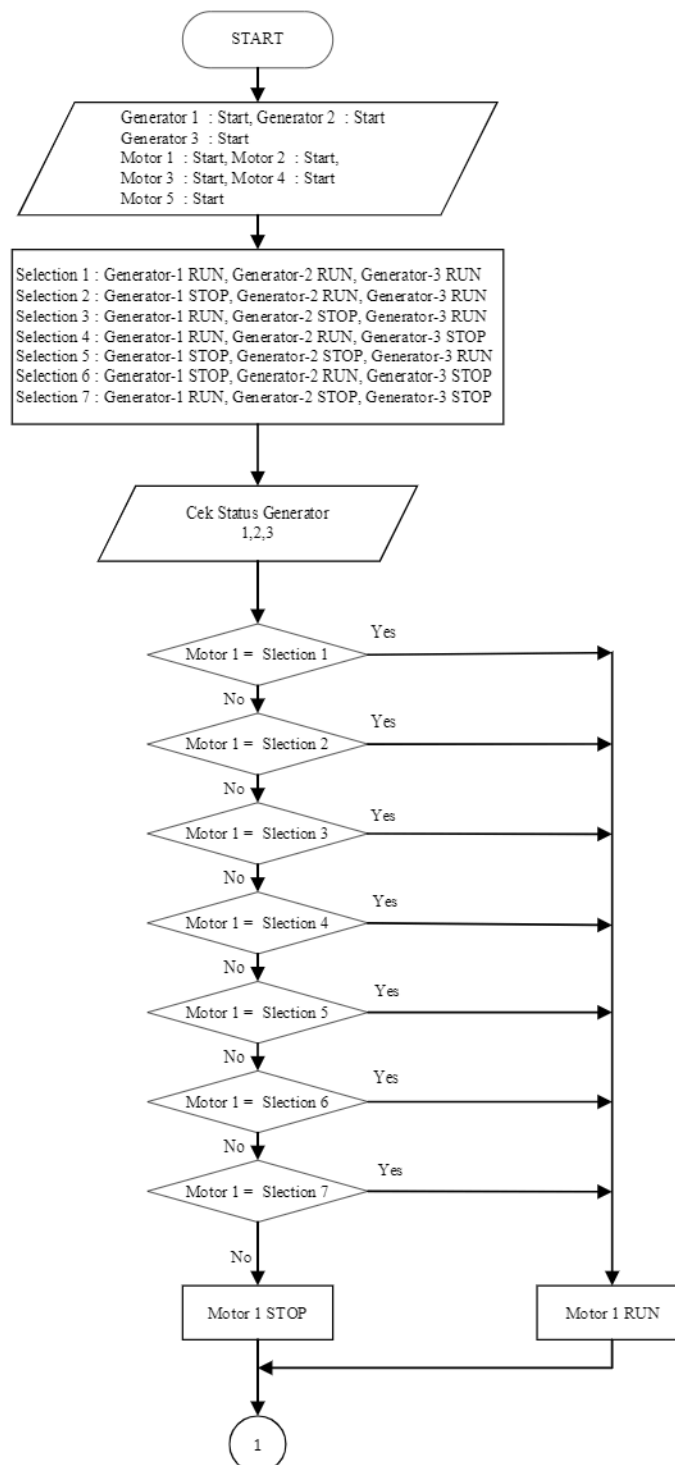
Figure 13. Flow chart diagram and logic program, for Motor-1.
