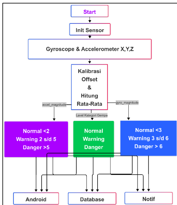
Gambar 1. Flowchart Proses Mitigasi Dini
