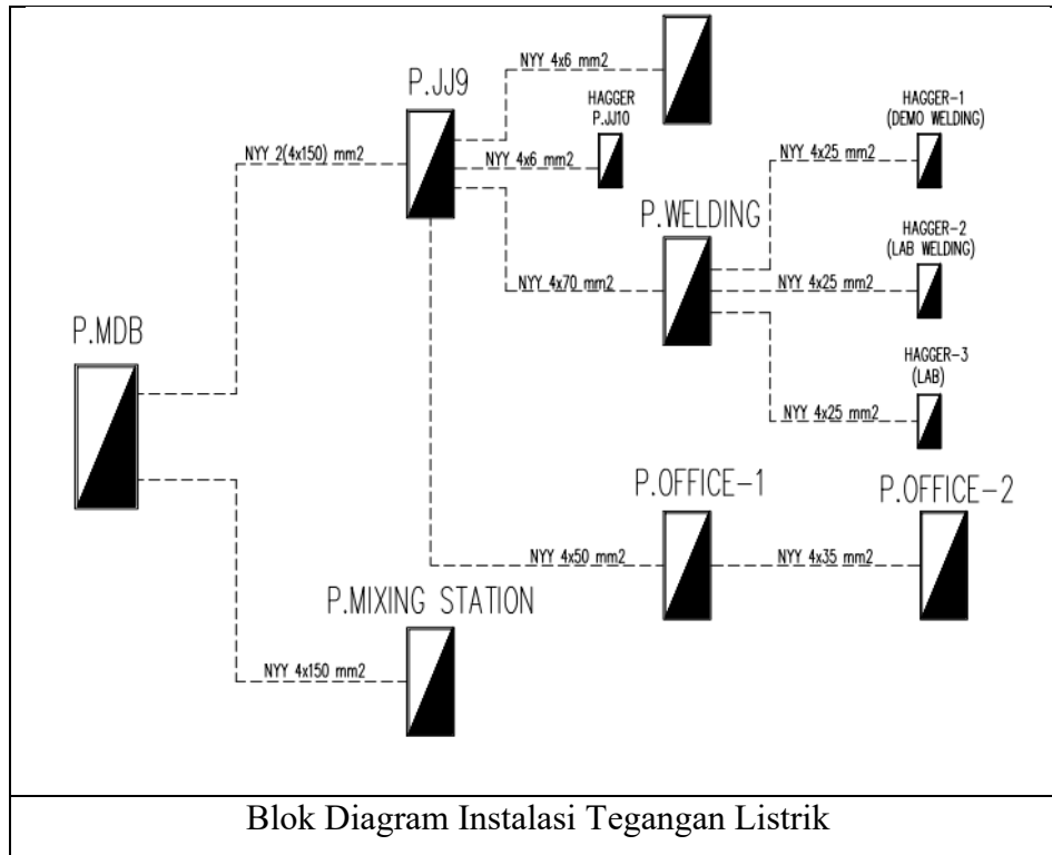
Gambar 4. 22 Blok Diagram Instalasi Tegangan Listrik PT. Voestalpine Bohler Welding Asia Pasific Sumber: Hasil Analisa
