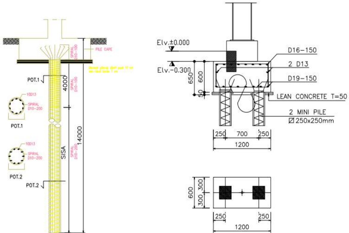
Gambar 4. 15 Detail Bore Pile Sumber: Hasil Analisa
