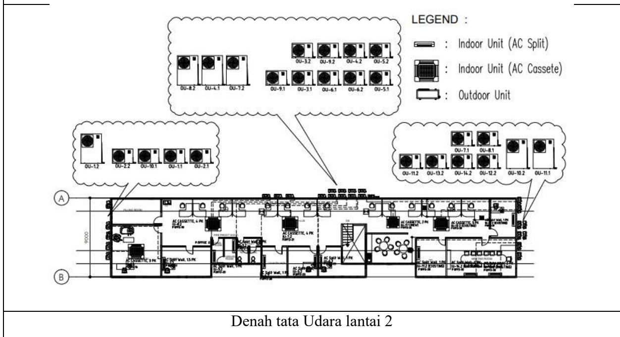
Gambar 4. 20 Denah tata udara PT. Voestalpine Bohler Welding Asia Pacific Sumber: Hasil Analisa
