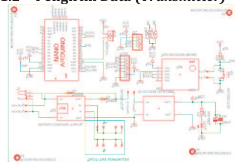
Gambar 17 Skema Wiring Diagram Transmitter
