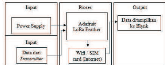
Gambar 16 Blok Diagram Receiver
