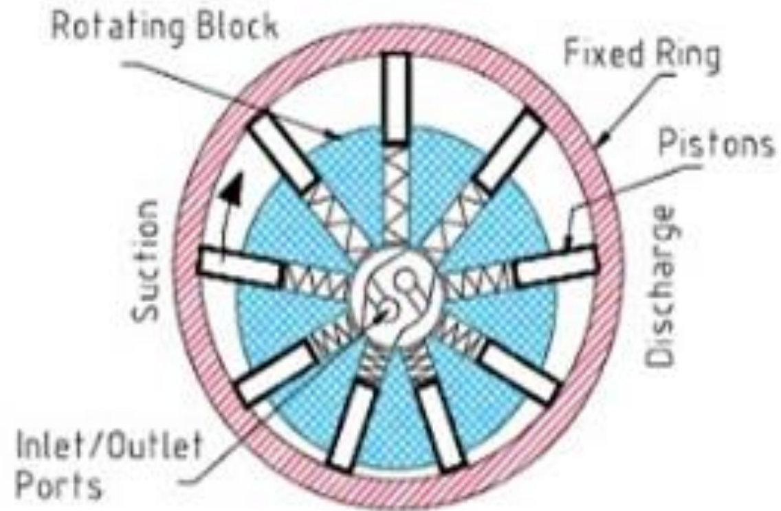
Radial Piston Pump
