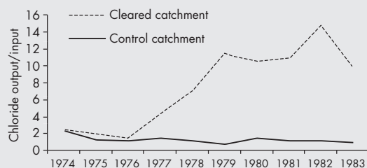
Figure 8.8 Chloride output/input ratio for two catchments in south-west Western Australia. These are the same two catchments as in Figures 8.6 and 8.7. Input has been measured through chloride concentrations in rainfall while output is streamflow.
