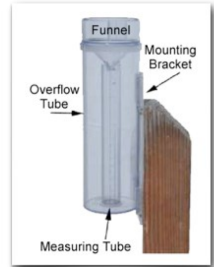
Components of a pole mounted standard rain gauge
