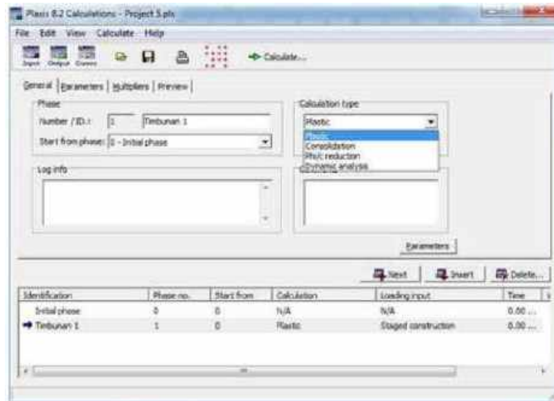
Gambar 2.38 Toolbar calculation
