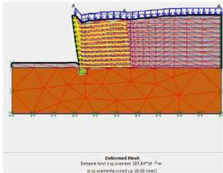
Gambar 2.39 Gambar contoh output Deformed Mesh
