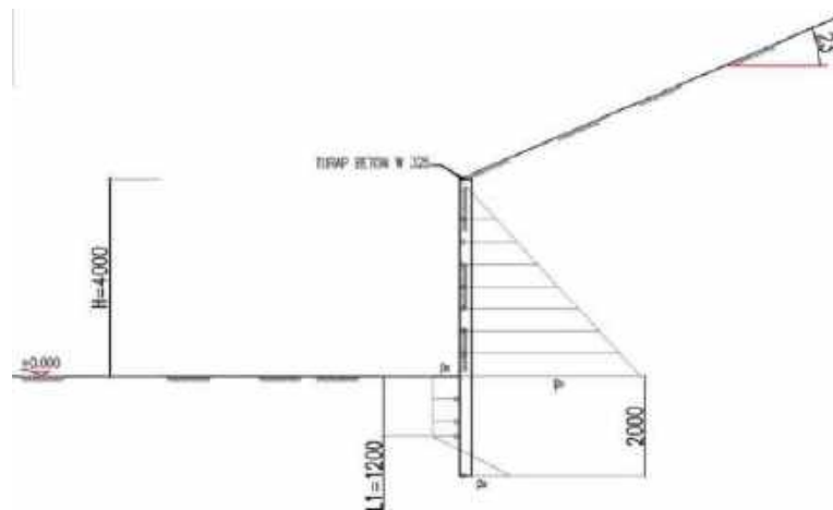
Gambar 4.12 Diagram tekanan tanah
