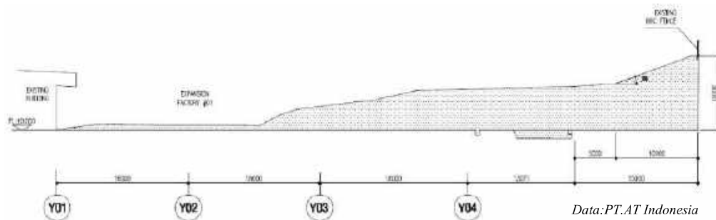
Gambar 3.2 Penampang lereng existing
