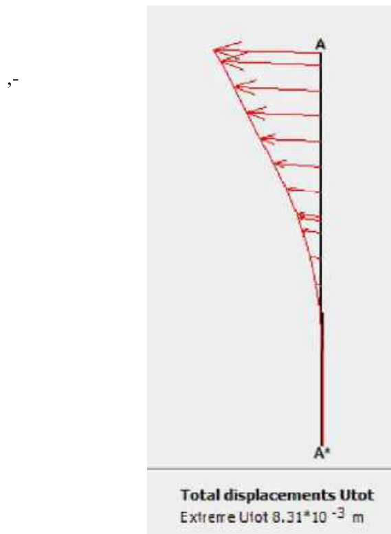
Gambar 4.26 Total Perpindahan borepile
