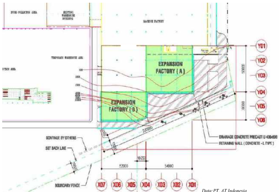
Gambar 3.1 Layout titik CPT-Boring test
