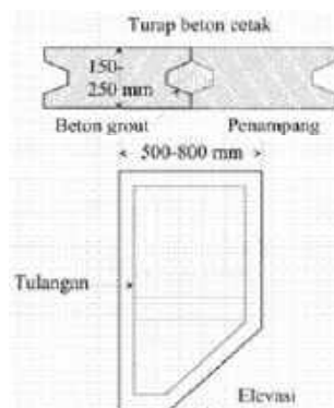
Gambar 2.19 Turap Beton Pracetak
