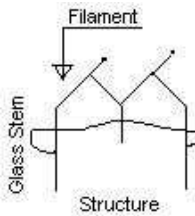
Figure 2 Directly Heated Cathode (DHC)
