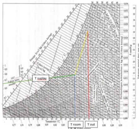
Gbr 4.1 Diagram Psycmetrik Sumber: ASHRAE HANBOOK 2021
